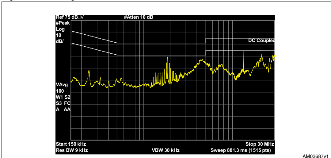
Figure 48. Average measurements at 230 Vac, full load
