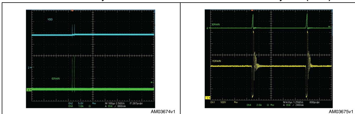
Figure 34. Operating with secondary winding shorted. Steady state
